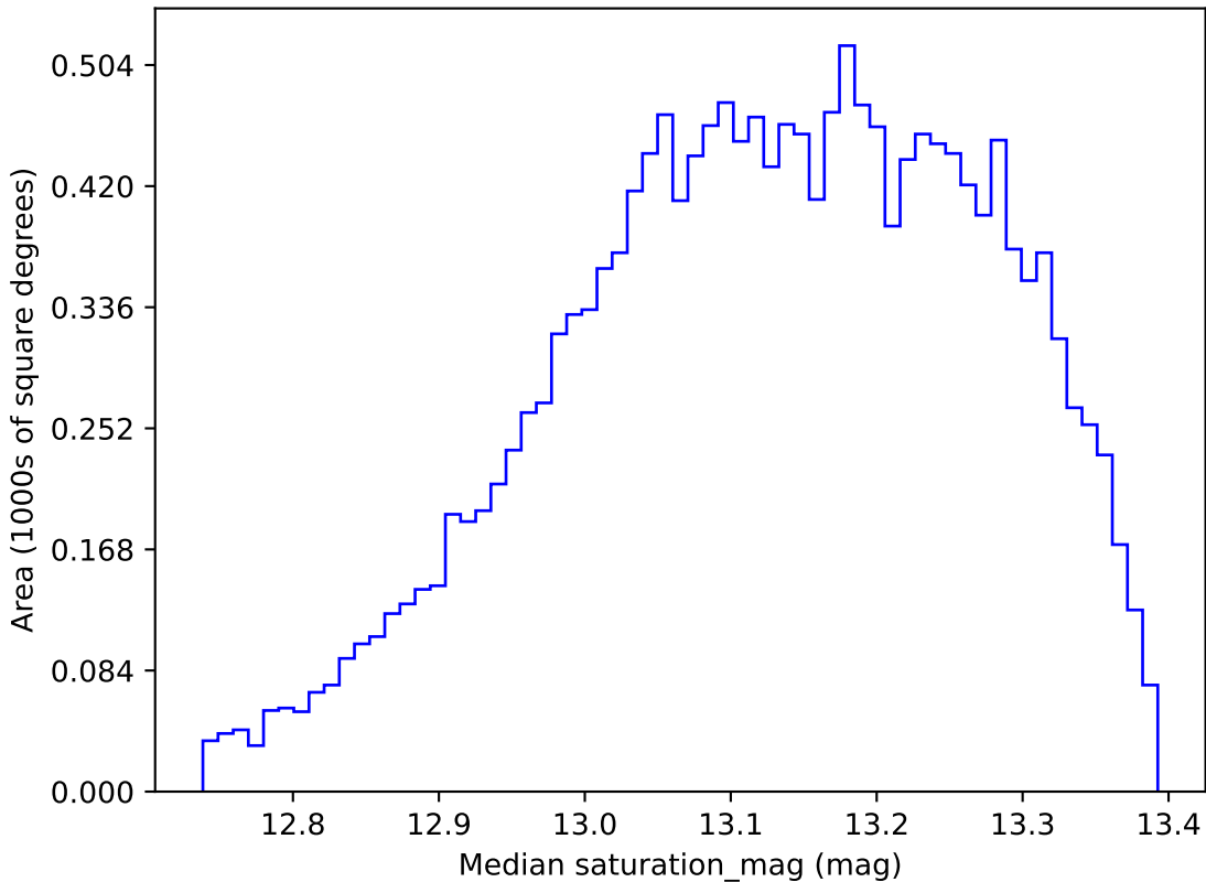
extra_ss_neo7_v3.4_10yrs WFD y band: Median saturation_mag
