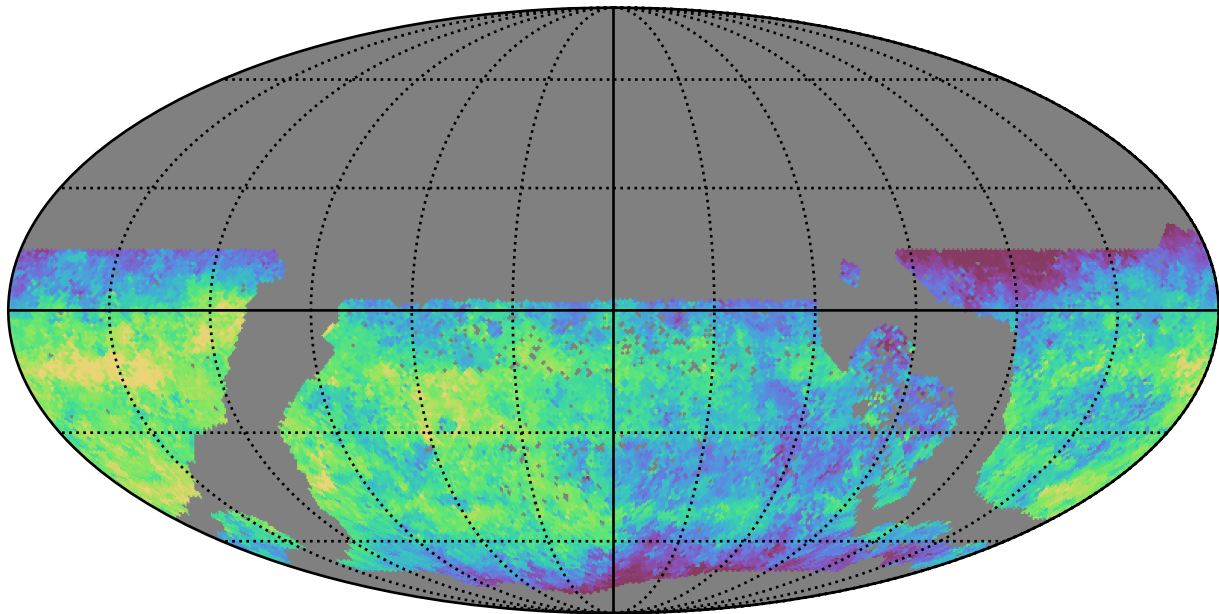
extra_ss_neo7_v3.4_10yrs WFD u band: Median saturation_mag
