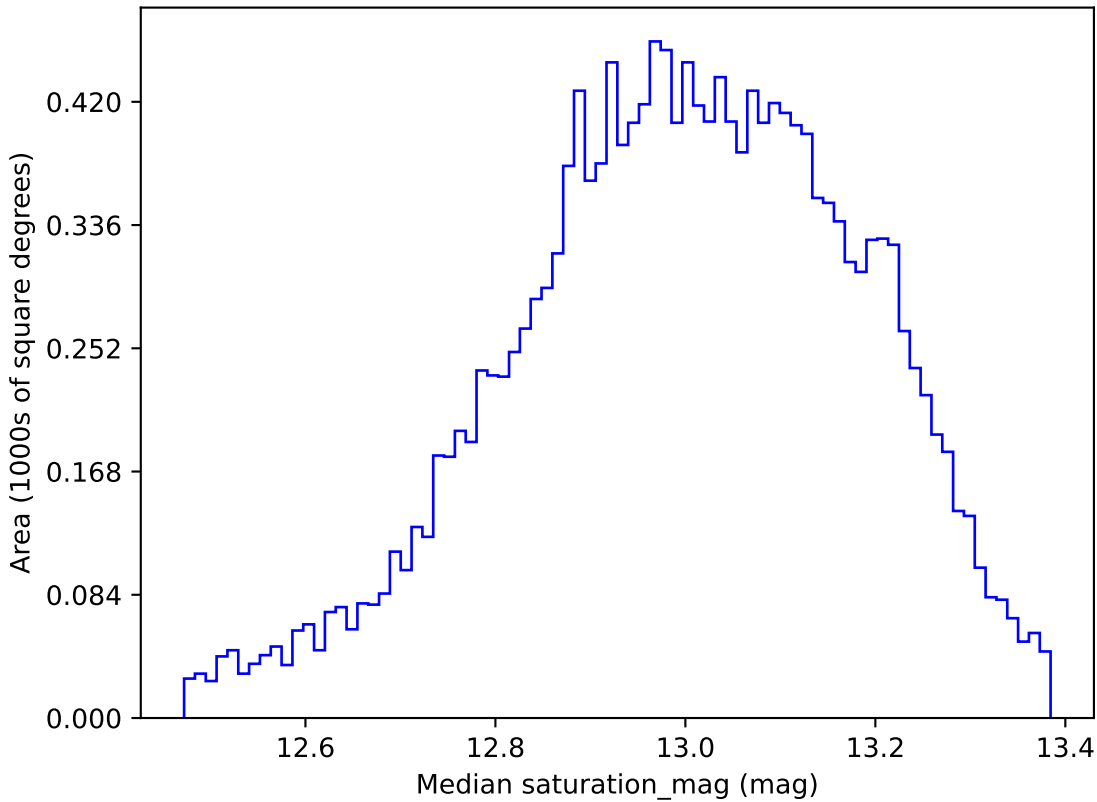
extra_ss_neo7_v3.4_10yrs WFD u band: Median saturation_mag
