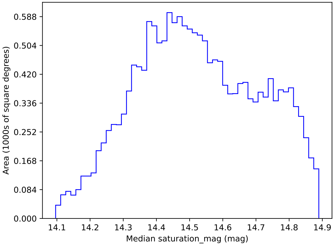
extra_ss_neo7_v3.4_10yrs WFD i band: Median saturation_mag
