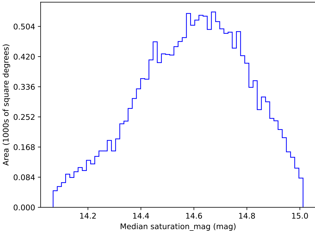
extra_ss_neo7_v3.4_10yrs WFD g band: Median saturation_mag
