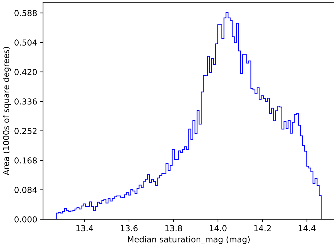
extra_ss_neo7_v3.4_10yrs All sky z band: Median saturation_mag
