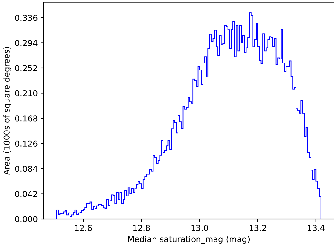
extra_ss_neo7_v3.4_10yrs All sky y band: Median saturation_mag
