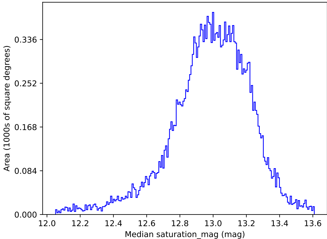
extra_ss_neo7_v3.4_10yrs All sky u band: Median saturation_mag
