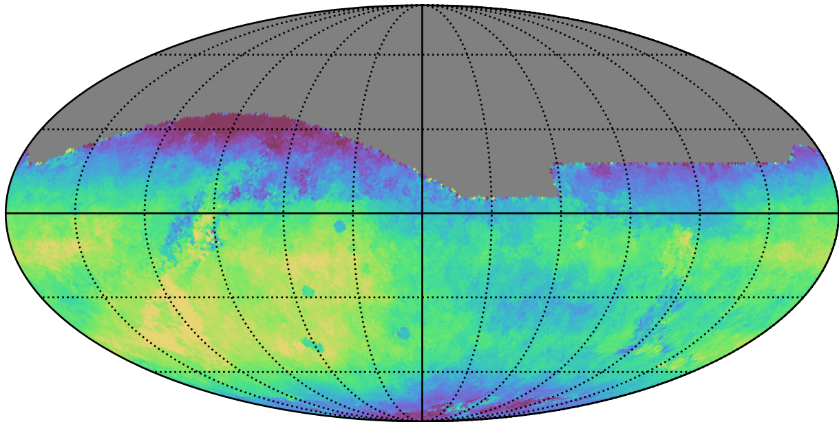
extra_ss_neo7_v3.4_10yrs All sky r band: Median saturation_mag
