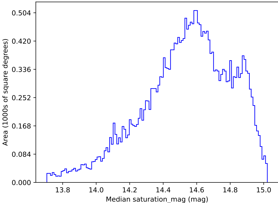
extra_ss_neo7_v3.4_10yrs All sky r band: Median saturation_mag
