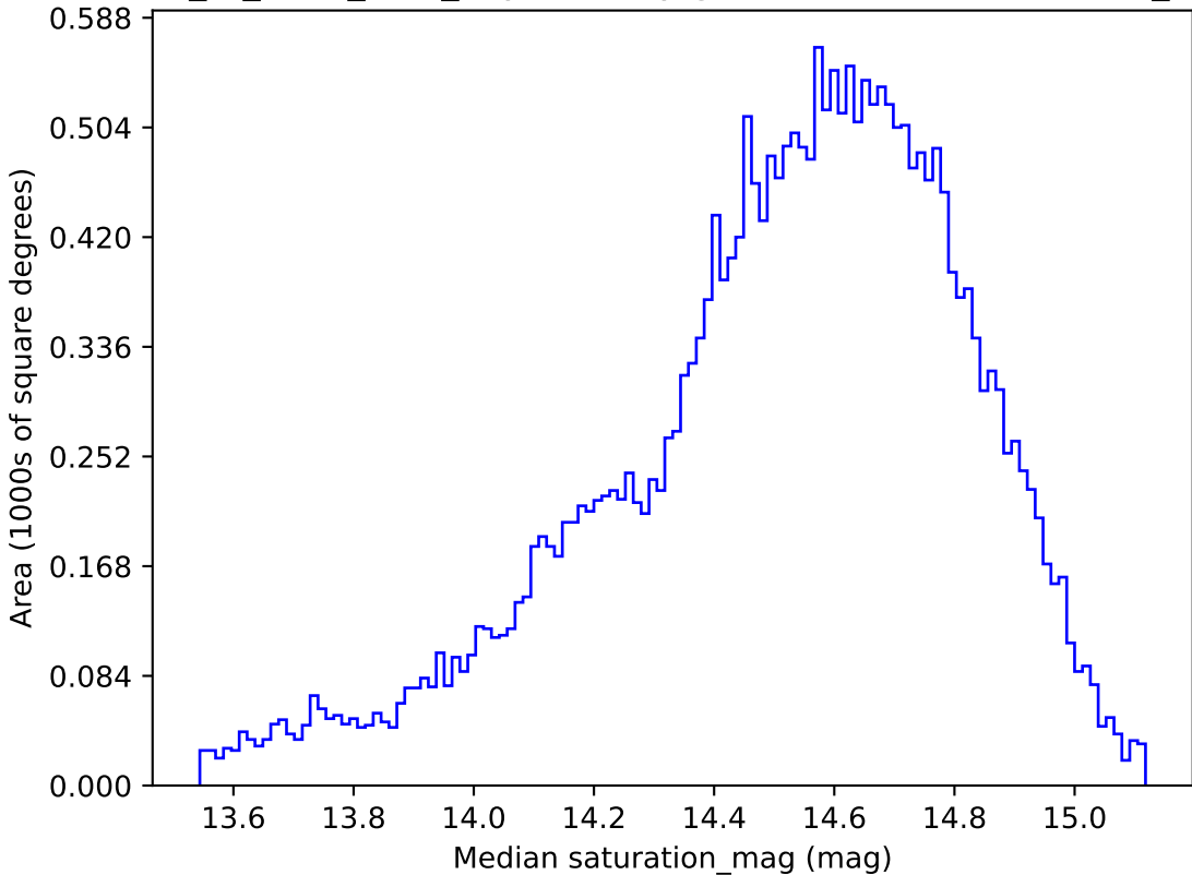
extra_ss_neo7_v3.4_10yrs All sky g band: Median saturation_mag
