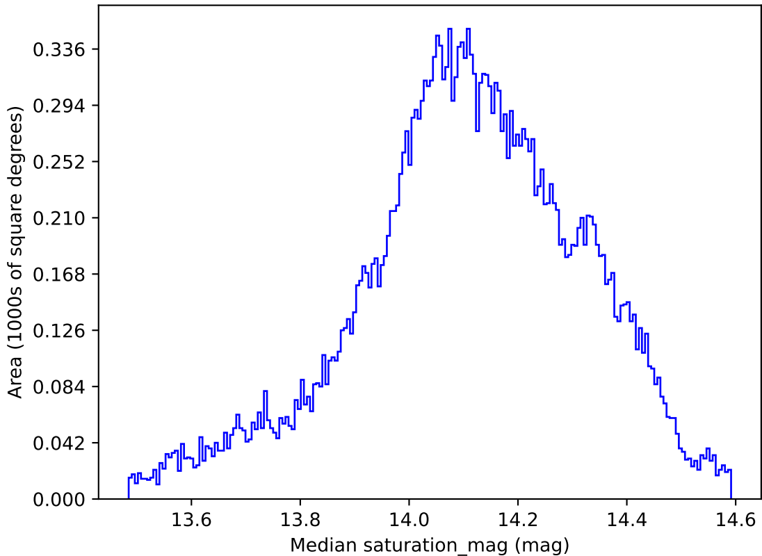
extra_ss_neo7_v3.4_10yrs All sky all bands: Median saturation_mag
