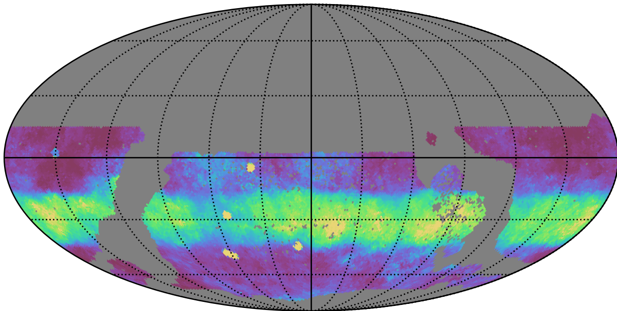
extra_ss_neo7_v3.4_10yrs WFD z band: Median normairmass
