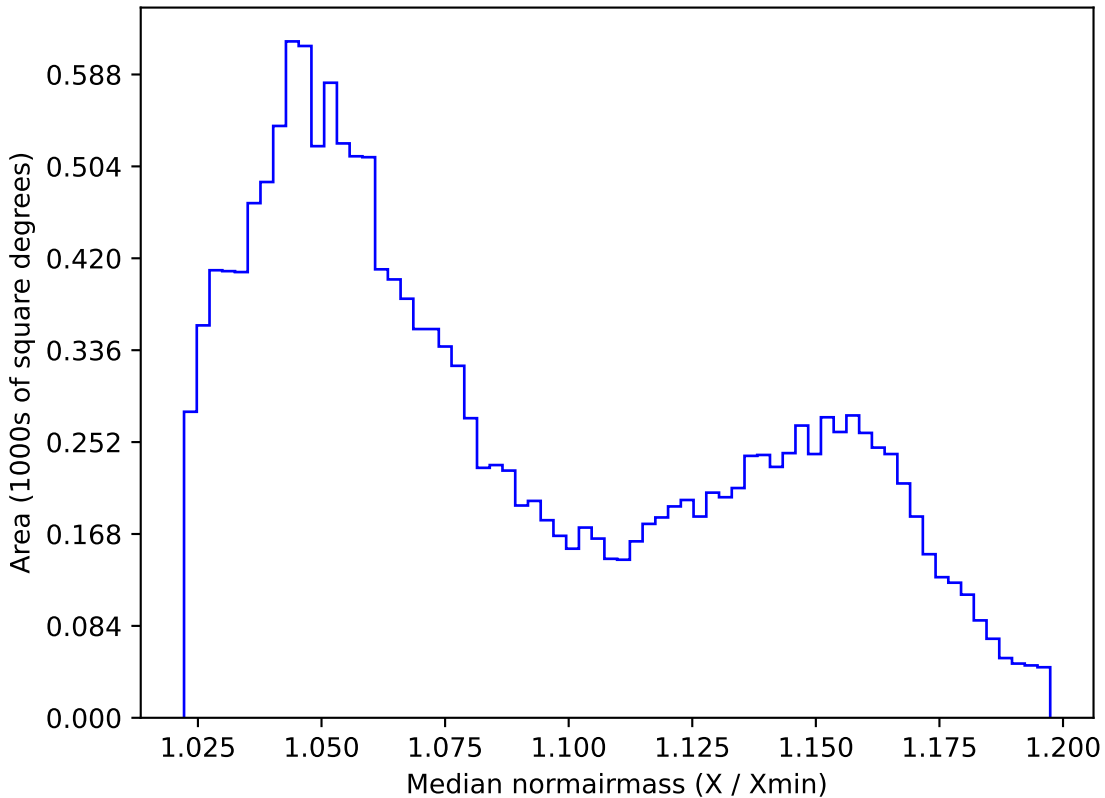
extra_ss_neo7_v3.4_10yrs WFD z band: Median normairmass
