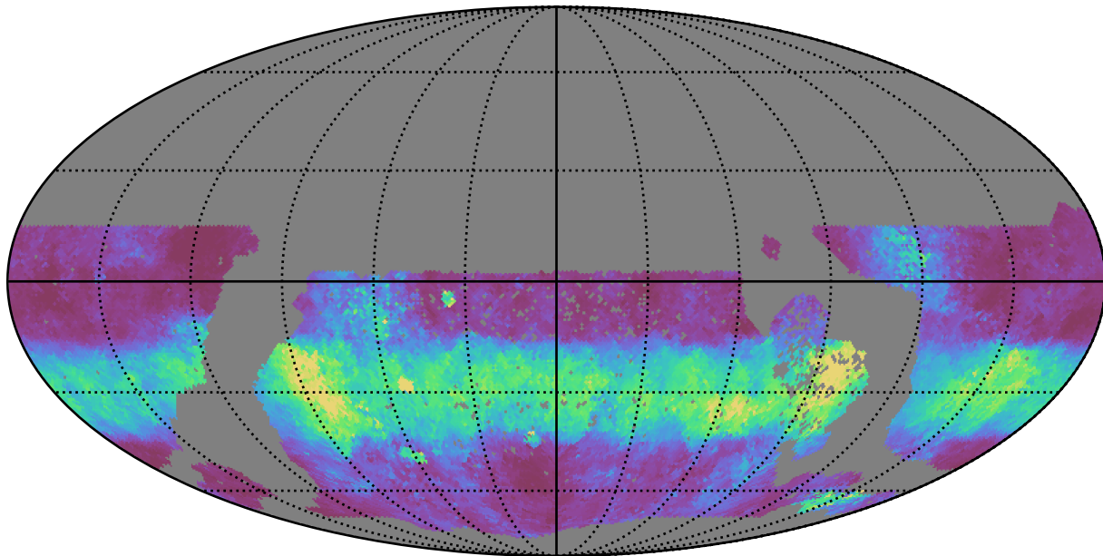
extra_ss_neo7_v3.4_10yrs WFD u band: Median normairmass
