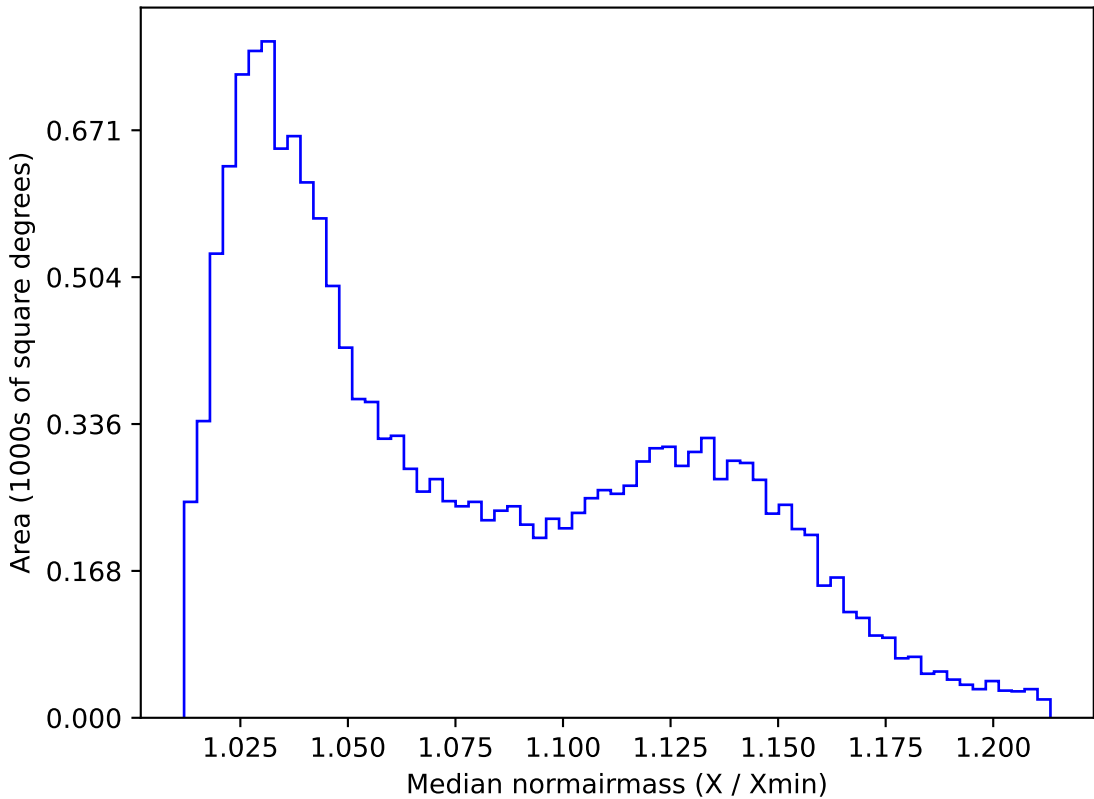
extra_ss_neo7_v3.4_10yrs WFD u band: Median normairmass
