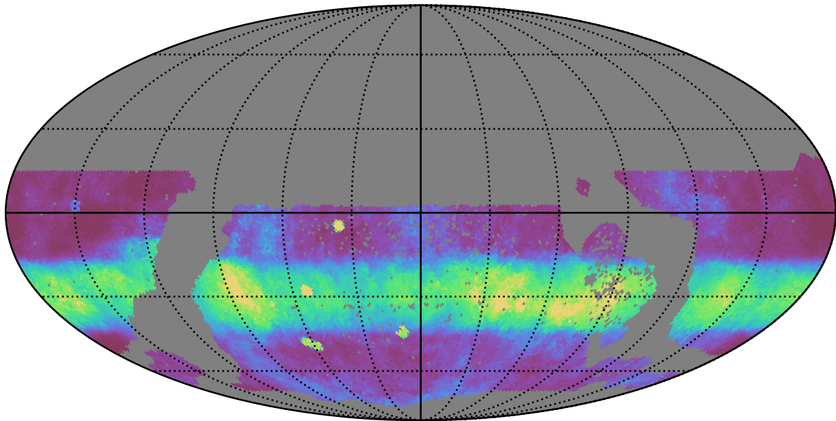
extra_ss_neo7_v3.4_10yrs WFD r band: Median normairmass
