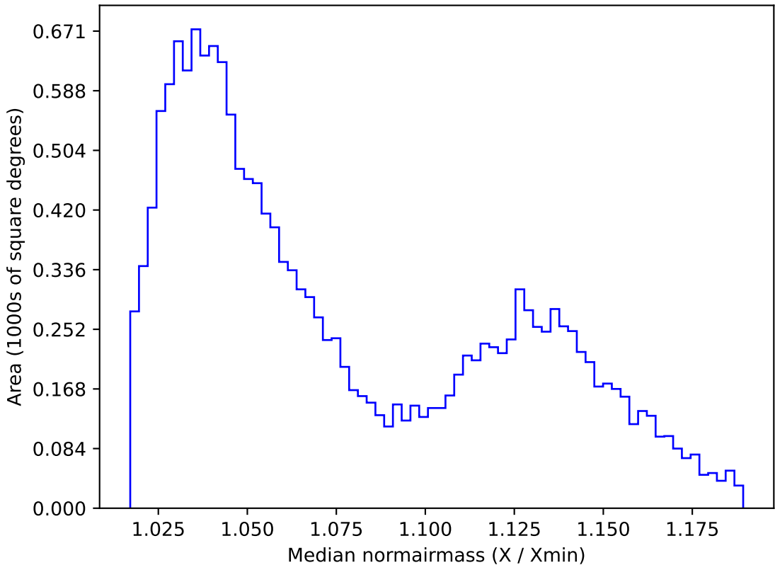
extra_ss_neo7_v3.4_10yrs WFD r band: Median normairmass
