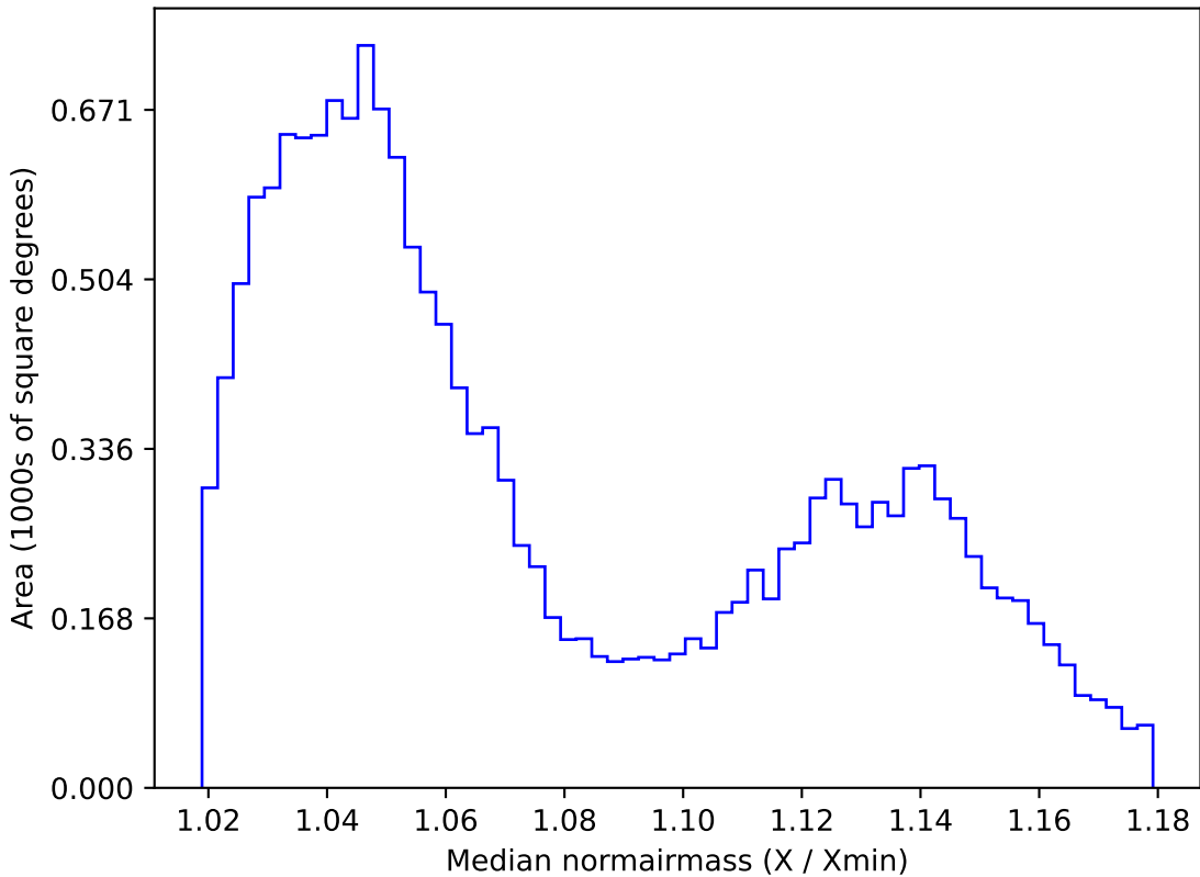
extra_ss_neo7_v3.4_10yrs WFD i band: Median normairmass
