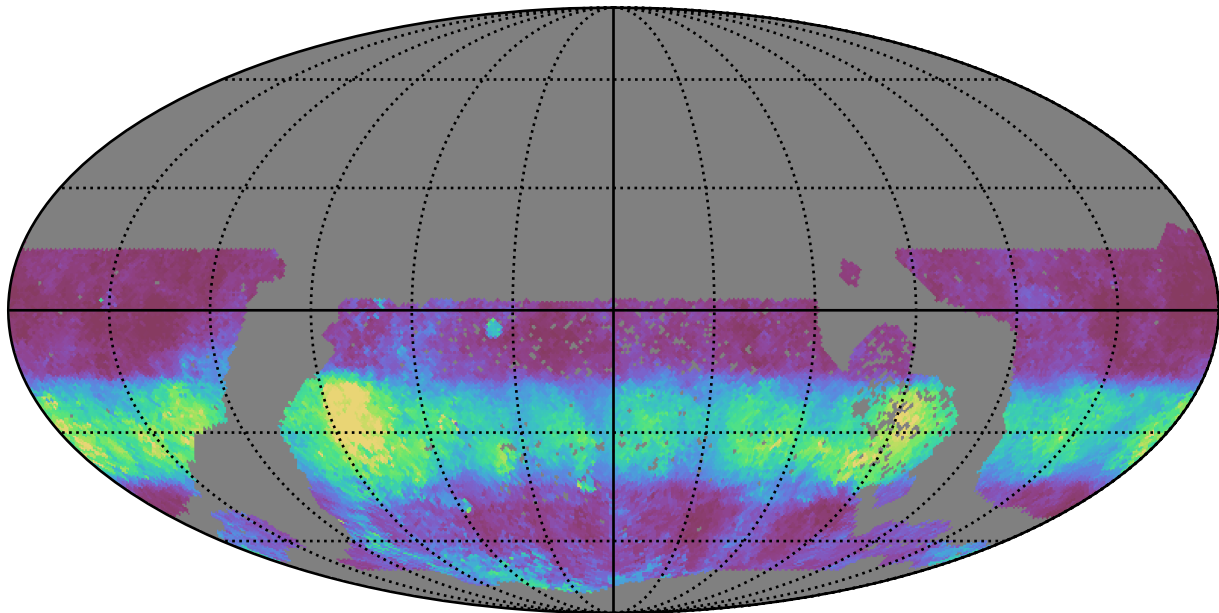
extra_ss_neo7_v3.4_10yrs WFD g band: Median normairmass
