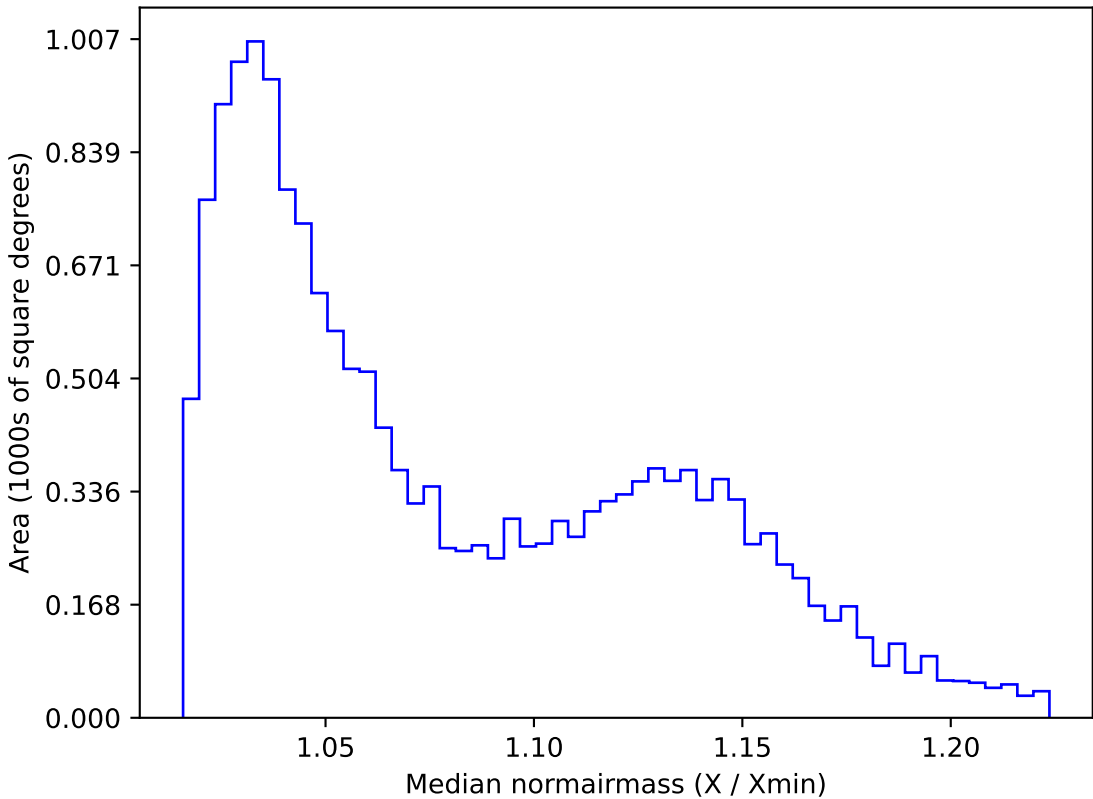
extra_ss_neo7_v3.4_10yrs WFD g band: Median normairmass
