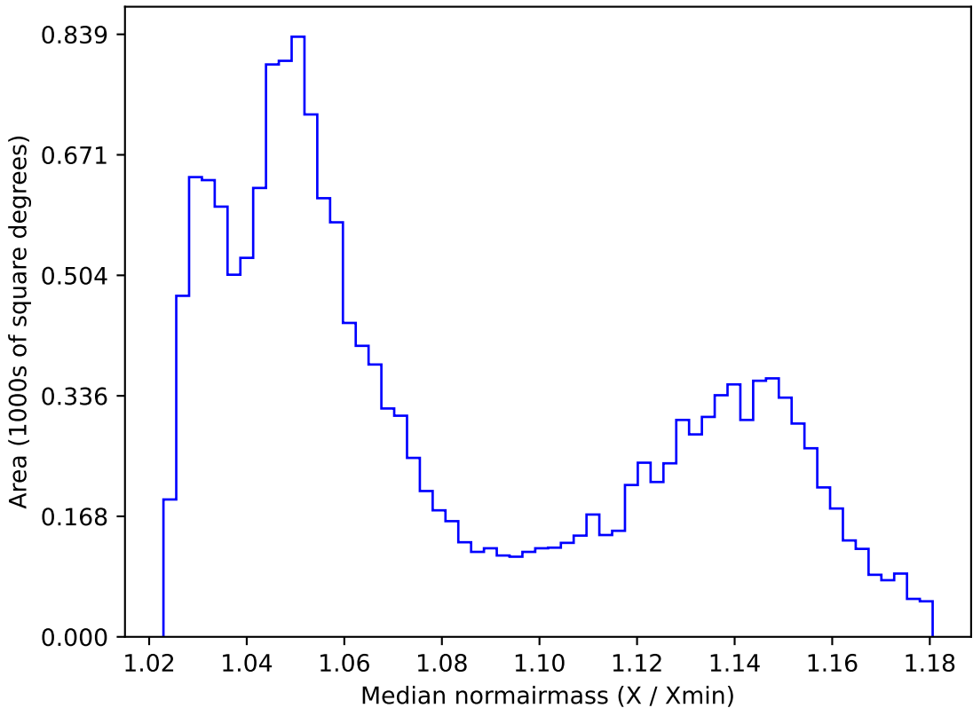
extra_ss_neo7_v3.4_10yrs WFD all bands: Median normairmass
