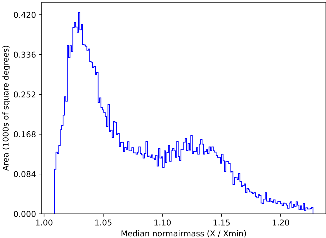
extra_ss_neo7_v3.4_10yrs All sky u band: Median normairmass
