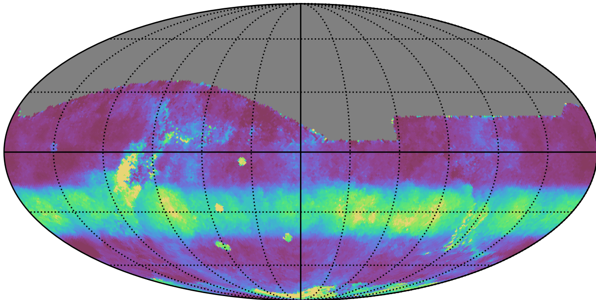
extra_ss_neo7_v3.4_10yrs All sky r band: Median normairmass
