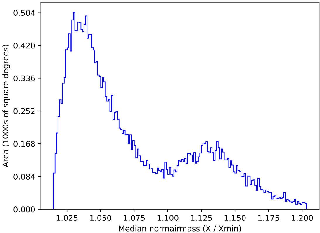
extra_ss_neo7_v3.4_10yrs All sky r band: Median normairmass
