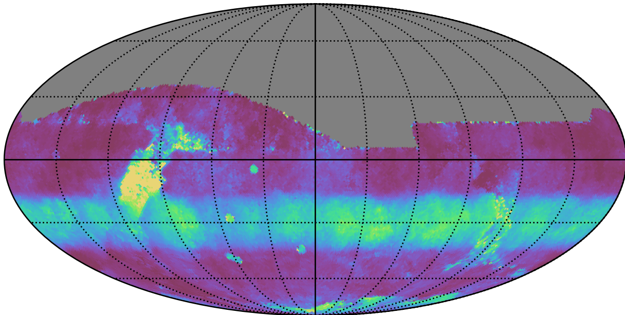
extra_ss_neo7_v3.4_10yrs All sky i band: Median normairmass
