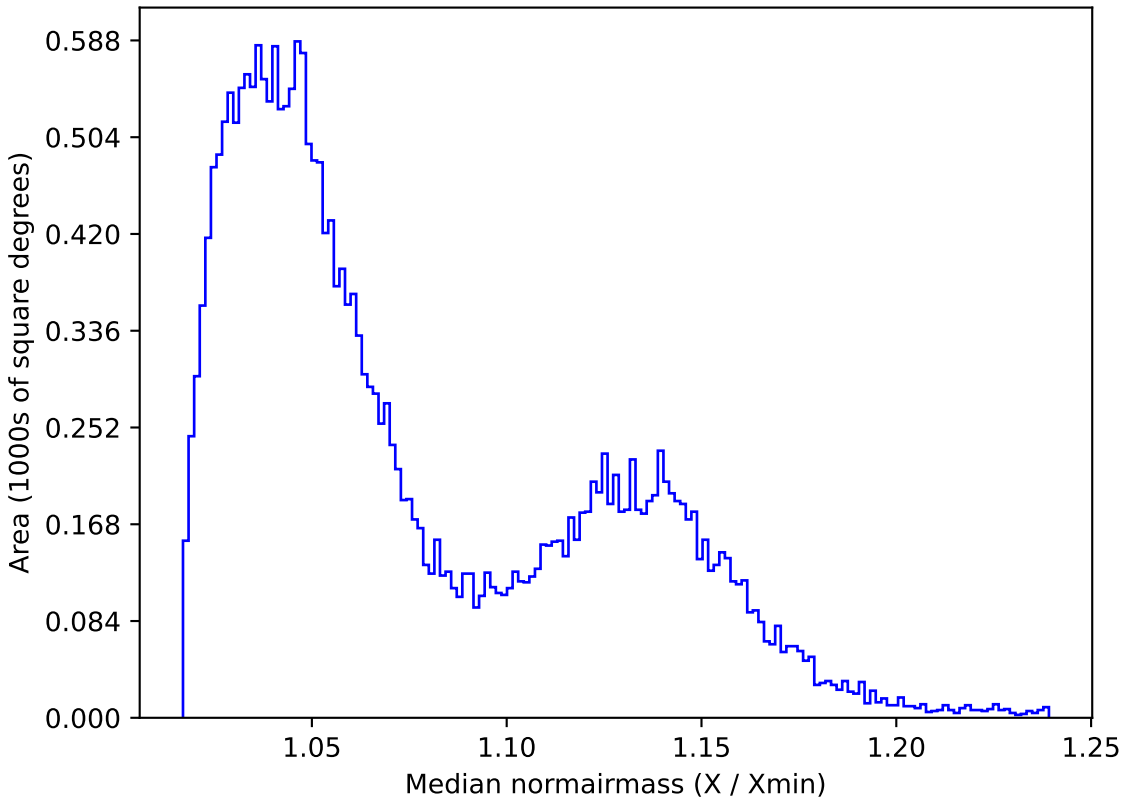
extra_ss_neo7_v3.4_10yrs All sky i band: Median normairmass
