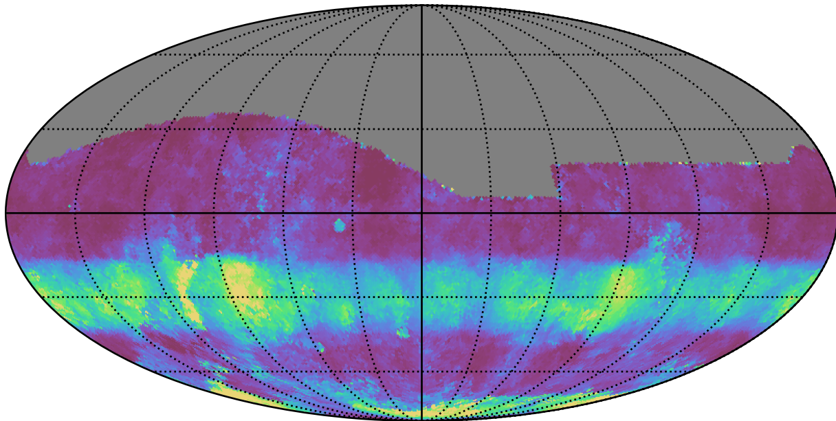
extra_ss_neo7_v3.4_10yrs All sky g band: Median normairmass
