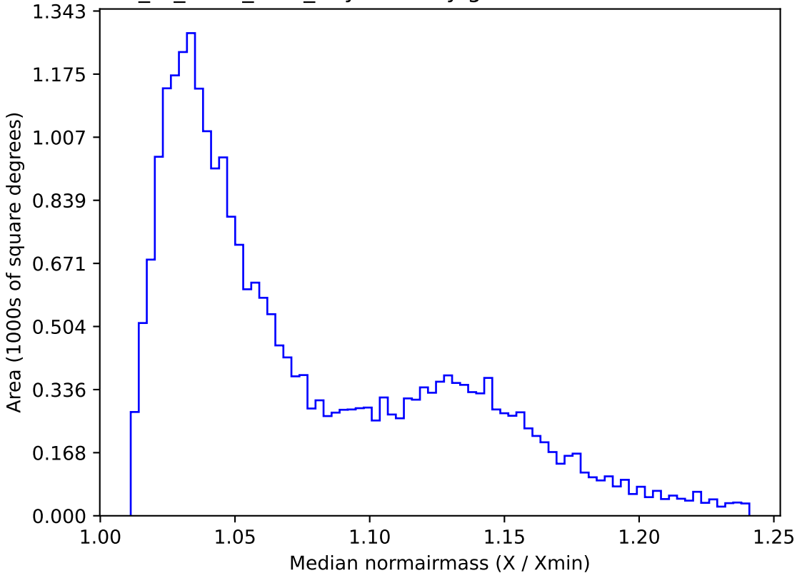
extra_ss_neo7_v3.4_10yrs All sky g band: Median normairmass
