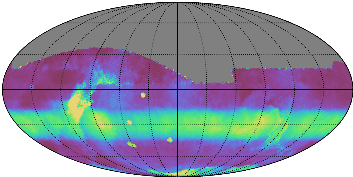
extra_ss_neo7_v3.4_10yrs All sky all bands: Median normairmass
