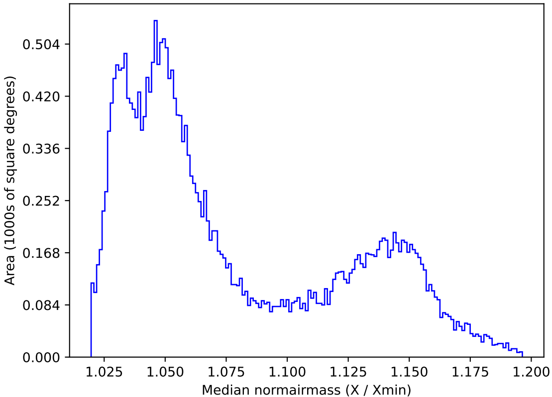
extra_ss_neo7_v3.4_10yrs All sky all bands: Median normairmass
