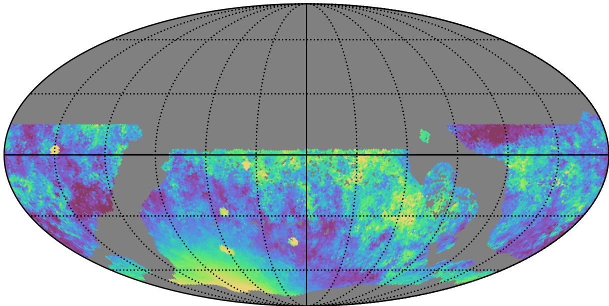
extra_ss_neo7_v3.4_10yrs WFD z band: Median moonDistance
