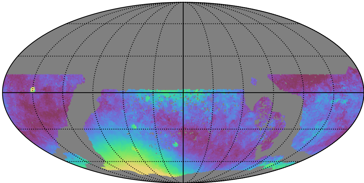
extra_ss_neo7_v3.4_10yrs WFD y band: Median moonDistance
