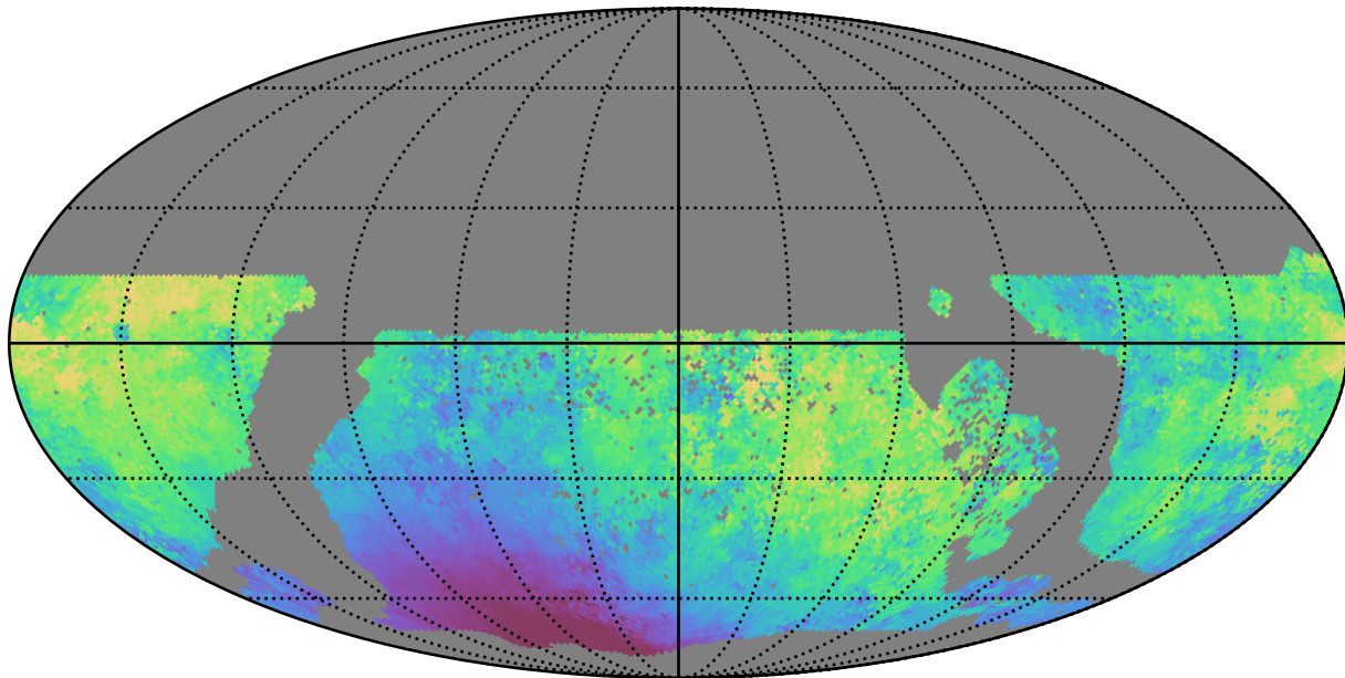
extra_ss_neo7_v3.4_10yrs WFD u band: Median moonDistance
