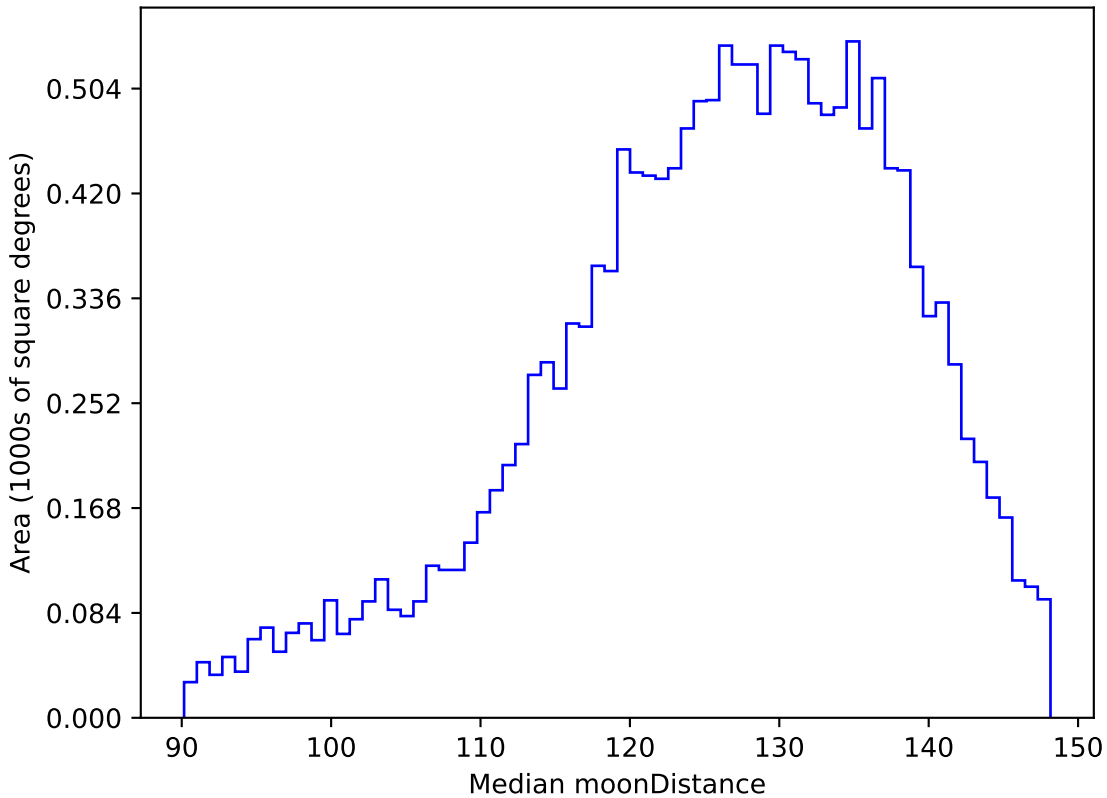
extra_ss_neo7_v3.4_10yrs WFD u band: Median moonDistance
