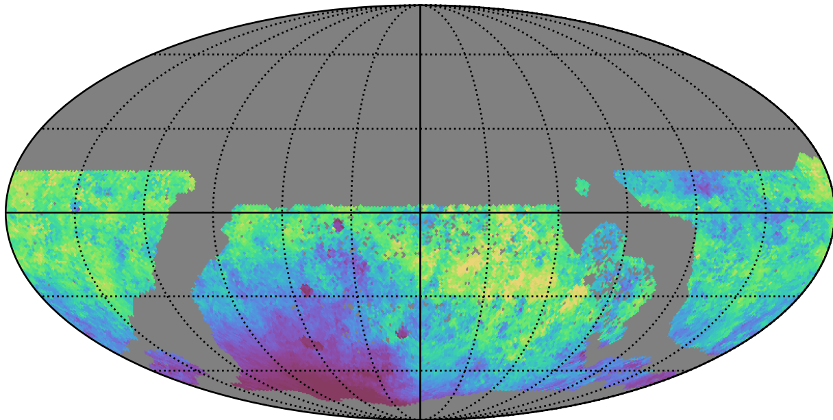
extra_ss_neo7_v3.4_10yrs WFD r band: Median moonDistance
