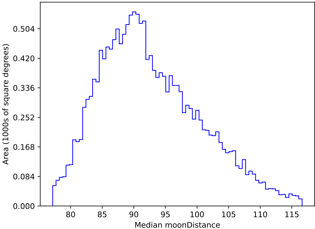
extra_ss_neo7_v3.4_10yrs WFD i band: Median moonDistance
