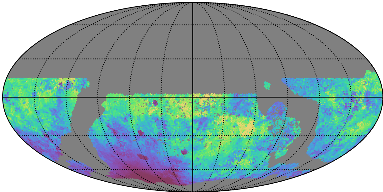
extra_ss_neo7_v3.4_10yrs WFD g band: Median moonDistance
