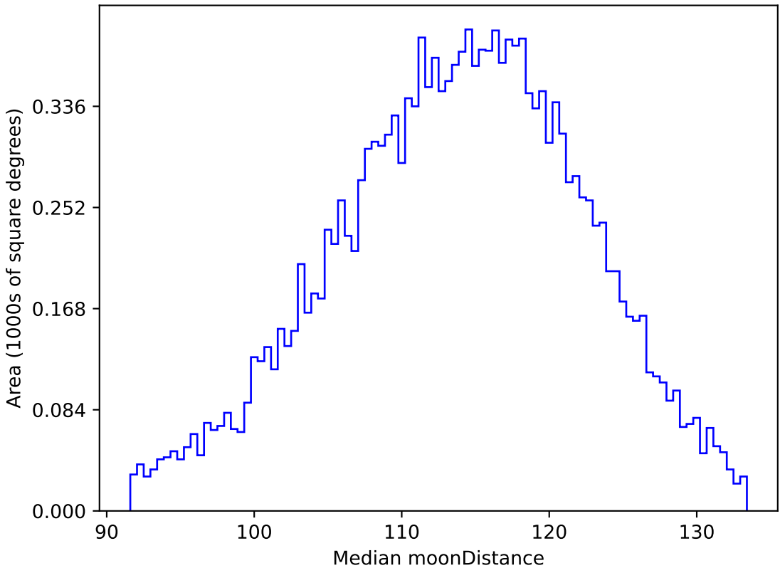
extra_ss_neo7_v3.4_10yrs WFD g band: Median moonDistance
