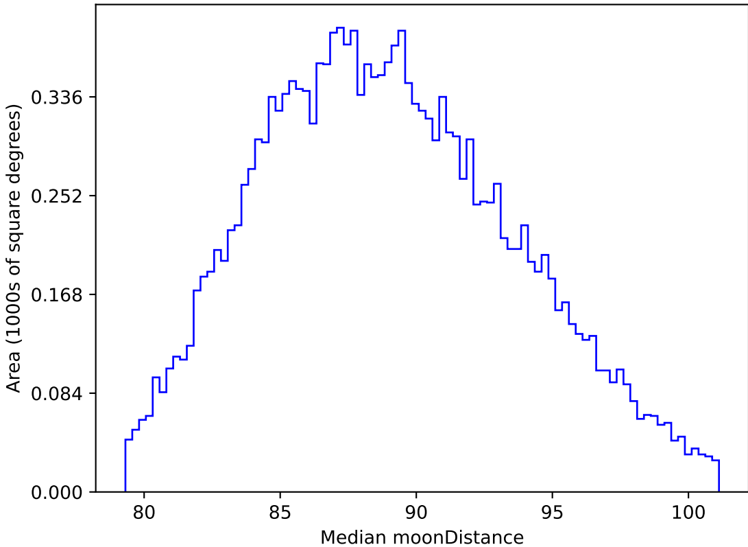
extra_ss_neo7_v3.4_10yrs WFD all bands: Median moonDistance
