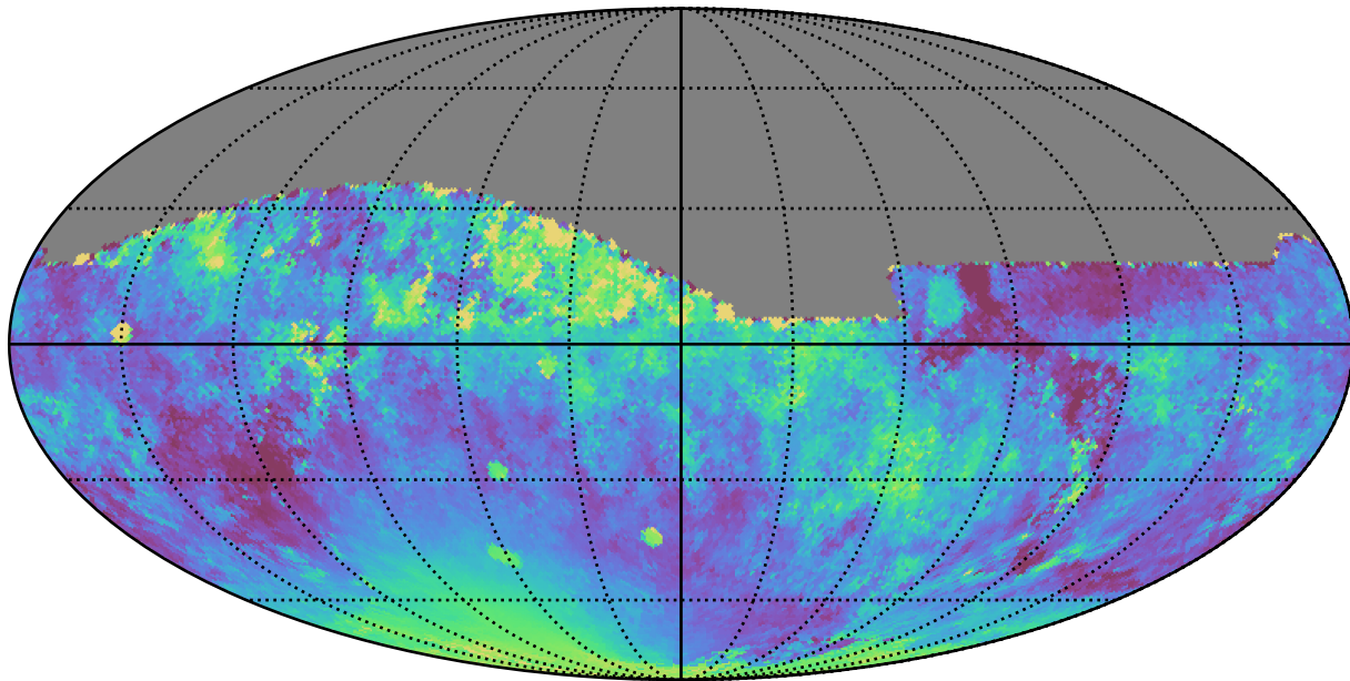
extra_ss_neo7_v3.4_10yrs All sky z band: Median moonDistance
