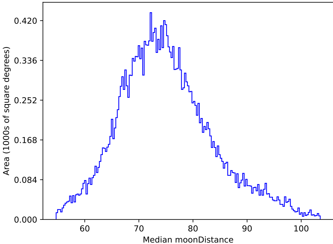
extra_ss_neo7_v3.4_10yrs All sky z band: Median moonDistance
