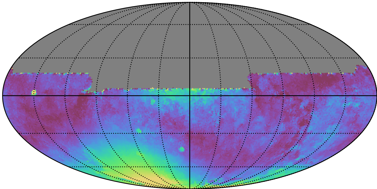
extra_ss_neo7_v3.4_10yrs All sky y band: Median moonDistance
