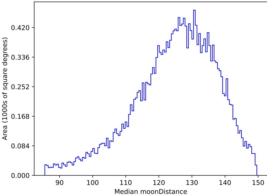
extra_ss_neo7_v3.4_10yrs All sky u band: Median moonDistance
