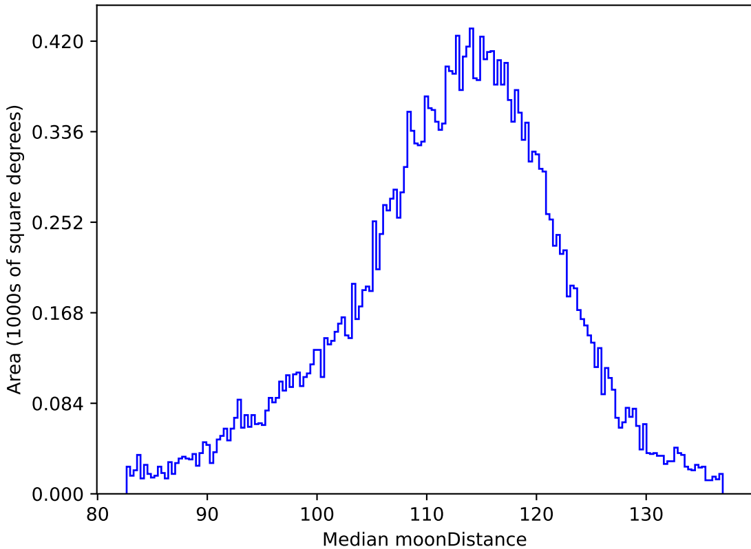
extra_ss_neo7_v3.4_10yrs All sky r band: Median moonDistance
