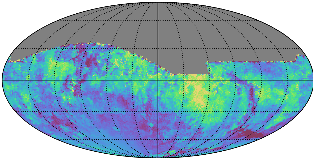
extra_ss_neo7_v3.4_10yrs All sky i band: Median moonDistance
