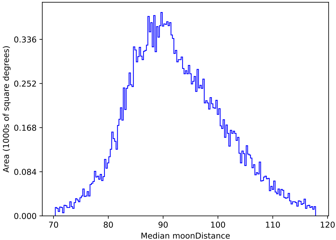
extra_ss_neo7_v3.4_10yrs All sky i band: Median moonDistance
