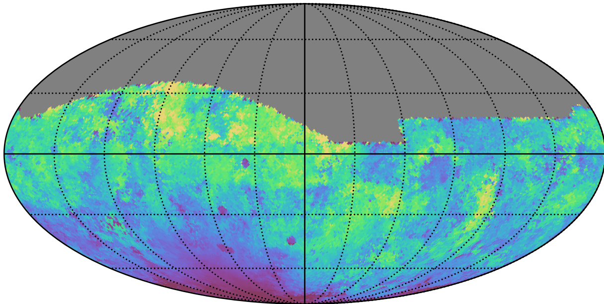
extra_ss_neo7_v3.4_10yrs All sky g band: Median moonDistance
