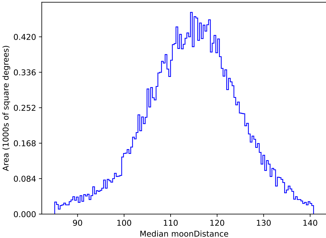
extra_ss_neo7_v3.4_10yrs All sky g band: Median moonDistance
