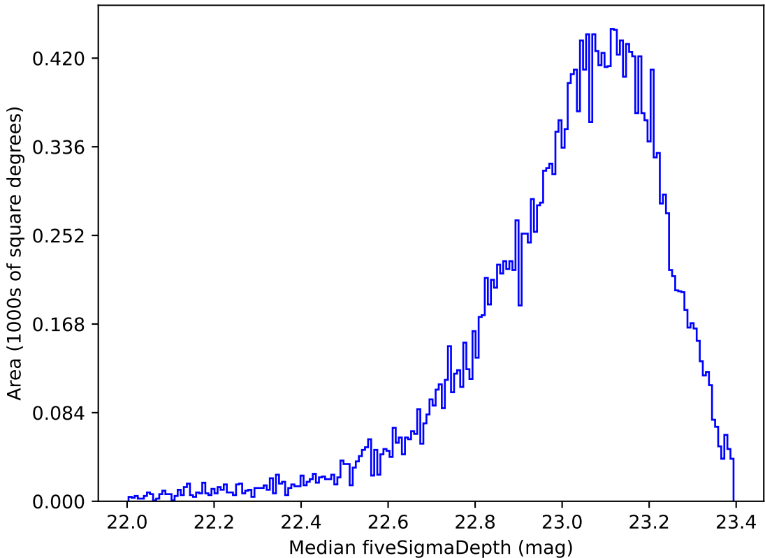
extra_ss_neo7_v3.4_10yrs Yr 1 z band: Median fiveSigmaDepth
